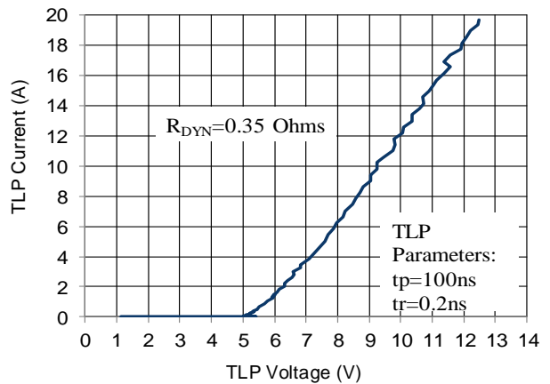
Figure 6: TLP Curve
