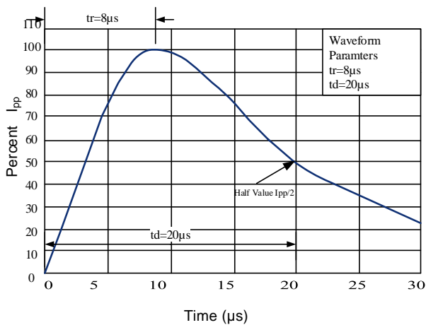
Figure 5: Pulse Waveform
